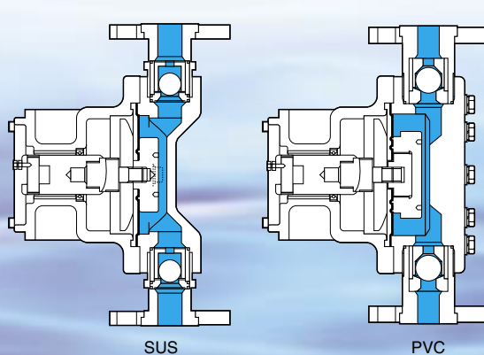
Mechanically-driven diaphragm
