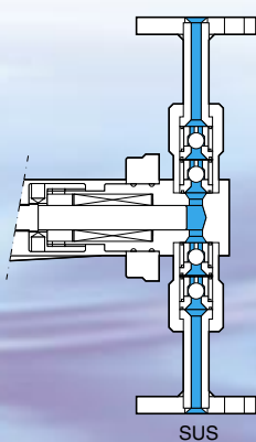
Plunger
