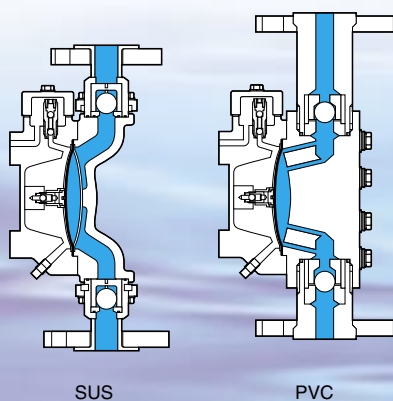
Hydraulic diaphragm
